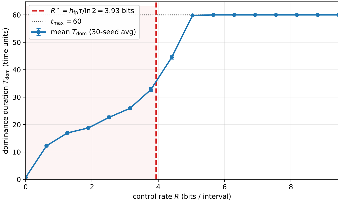
Entropy gap bounds dominance duration (Lorenz-96, N = 20 , F = 8 )
